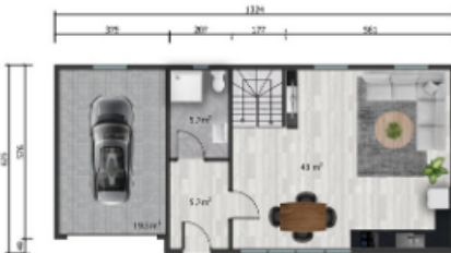
Zemin kat planı/ Ground floor plan
